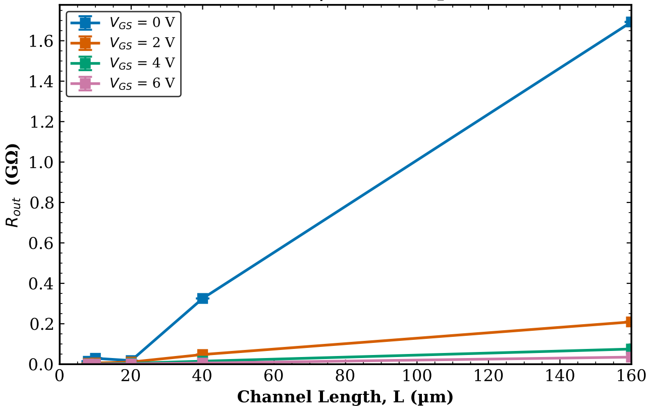
TFT1 Transistor 1 R_{out} vs L | W = 100\text{ }\mu\text{m}
